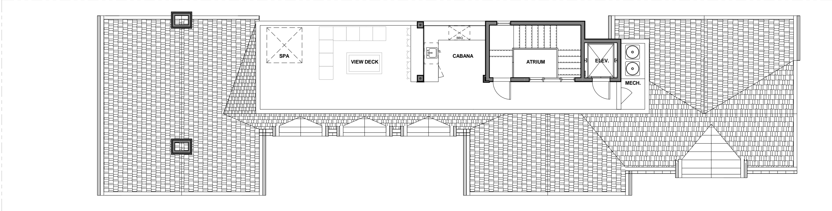
THIRD FLOOR PLAN 600 ACACIA SC. 1/8"=1'-0" THIRD FLOOR - 11 SF
